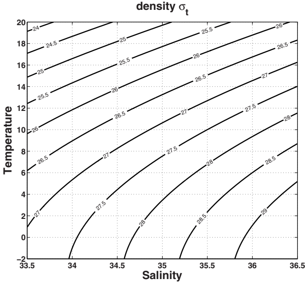
Figure 1.8. Contour plot of the density \sigma_t versus temperature T and salinity S using the UNESCO formula (Fofonoff and Millard, 1983).
