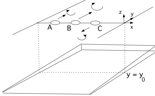
Figure 7.6. Propagation mechanism of Rossby waves in a layer of liquid on a sloping bottom.
