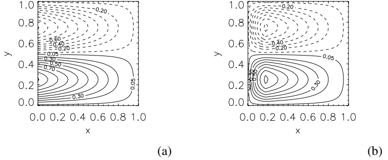
Figure 6.4. (a) Sverdrup flows for the wind stress field \tau^x(x, y) = -1/(2\pi) \cos 2\pi y , \tau^y(x, y) = 0 . (b) Total flow solution with Stommel western boundary current for \delta_S/L = 0.1 .
