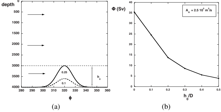
Figure 14.5. (a) Plot of the bottom topography versus the parameter h_0/D for \delta = 10^\circ . (b) Plot of the channel transport \Phi versus h_0/D for A_H = 2.5 \times 10^5 \text{ m}^2/\text{s} .
