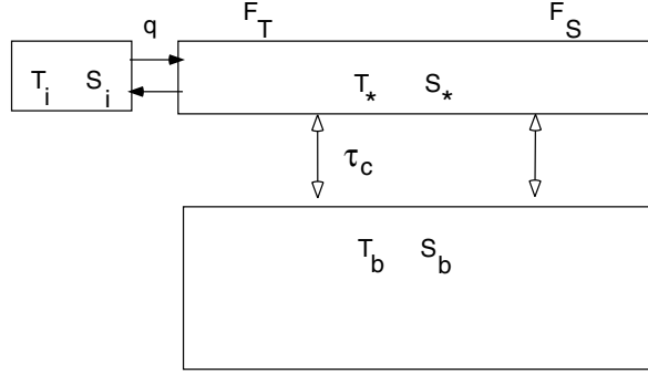
Figure 16.10. Sketch of the box model set-up to illustrate the convective feedback. An active box of temperature T_* , S_* is coupled to boxes of constant temperature T_i , S_i and T_b , S_b . Advective exchange takes place with flow rate q and vertical (convective) exchange occurs, on a time scale \tau_c , if the surface water is denser than the bottom water.
