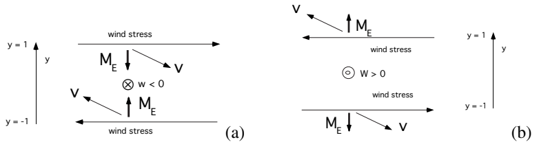
Figure 5.12. Example of Ekman (a) pumping ( \gamma > 0 ) and (b) suction ( \gamma < 0 ) caused by (a) a convergence and (b) a divergence of mass in the surface Ekman layer.
