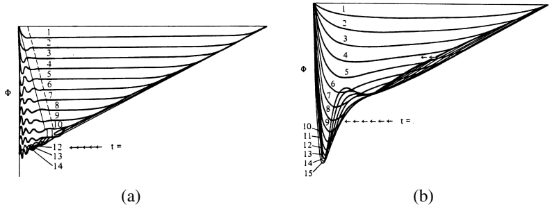
Figure 9.6. Adjustment for (a) \tilde{\Lambda} = 600 and (b) \tilde{\Lambda} = 20 . The labels at the curves mark subsequent time steps (from Anderson and Gill (1975)).
