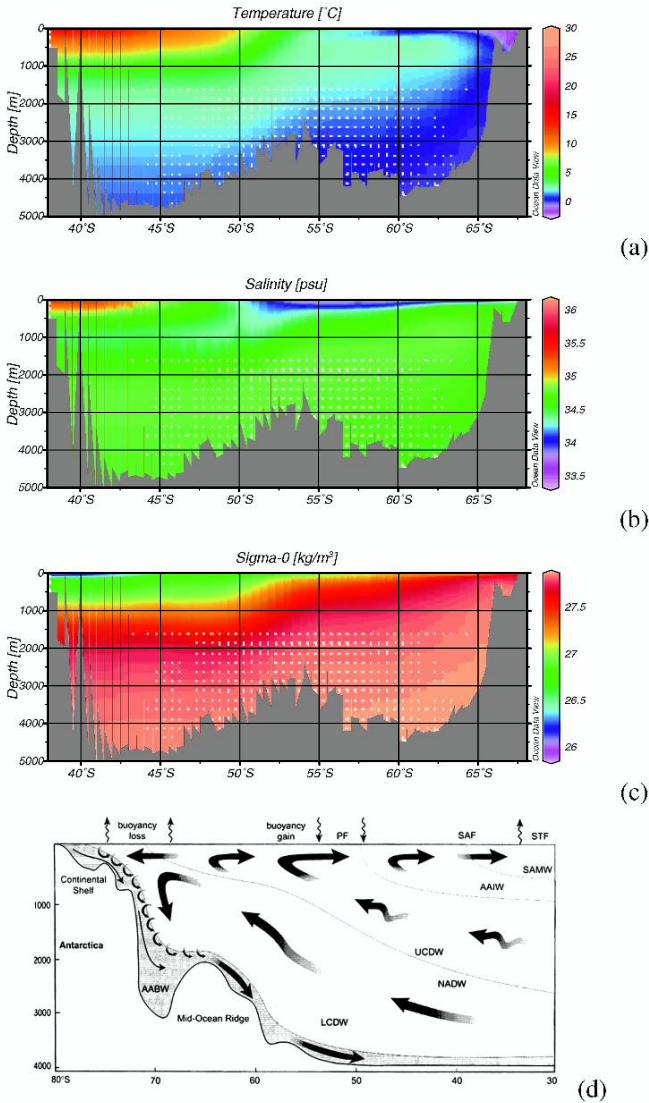
Figure 14.3. Profiles of temperature (a), salinity (b) and (c) potential density \sigma_0 along the WOCE 140°E meridional section; note that in all panels south is to the right. (d) Sketch of the zonally averaged circulation in the Southern Ocean; note that south is to the left (from WOCE (2001)).
