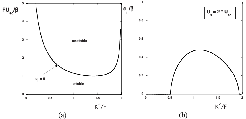
Figure 10.10. (a) Plot of the critical value of U_{sc} from (10.62). Note that with y = U_{sc}F/\beta and x = K^2/F , here the function y = 2/(x\sqrt{4-x^2}) is plotted. (b) The growth factor c_i from (10.61) for U_s = 2\beta/F ; with y = c_i/\beta and x = K^2/F here the function y = \sqrt{x^2(4-x^2)} - 1/(x^2+2) is plotted.
